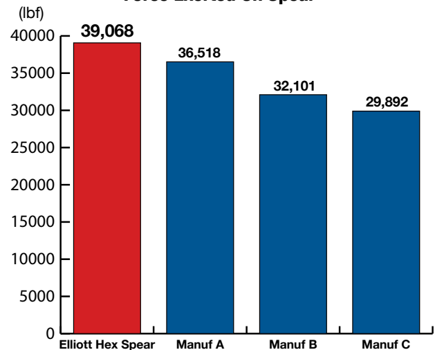
Force Exerted On Spear
