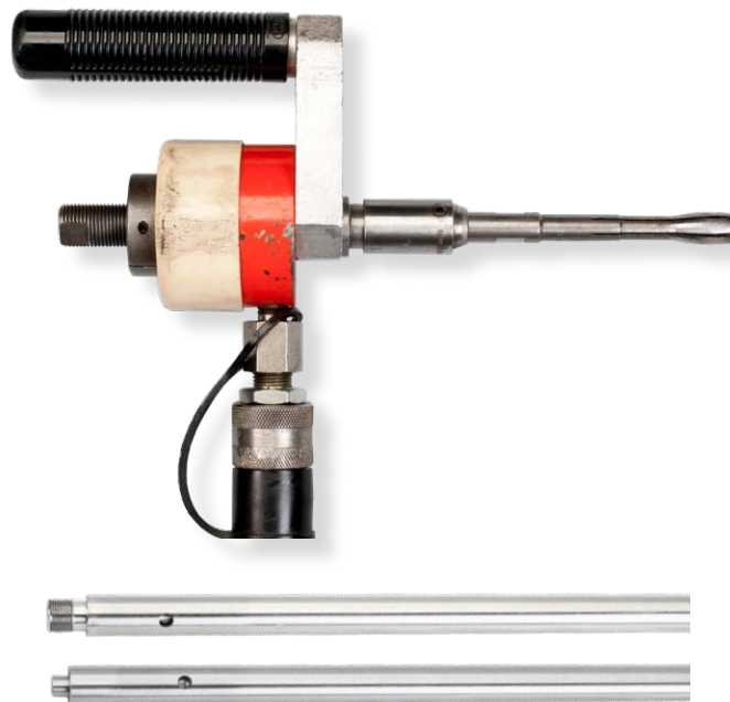
Collet Extensions
